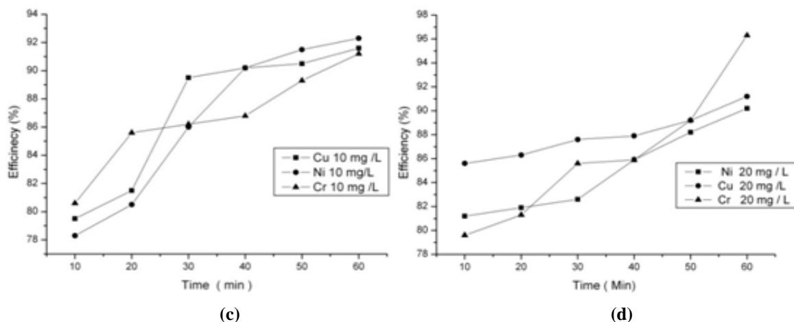
Figure 4: Removal Efficiency of Heavy Metals Adsorbed by Olive Oil Stabilized MIONS (a) & (b) and Flaxseed Oil Stabilized MIONS (c) and (d) for 10 mg/L and 20 mg/L Concentrations as a Function of Contact Time at pH 2.5
