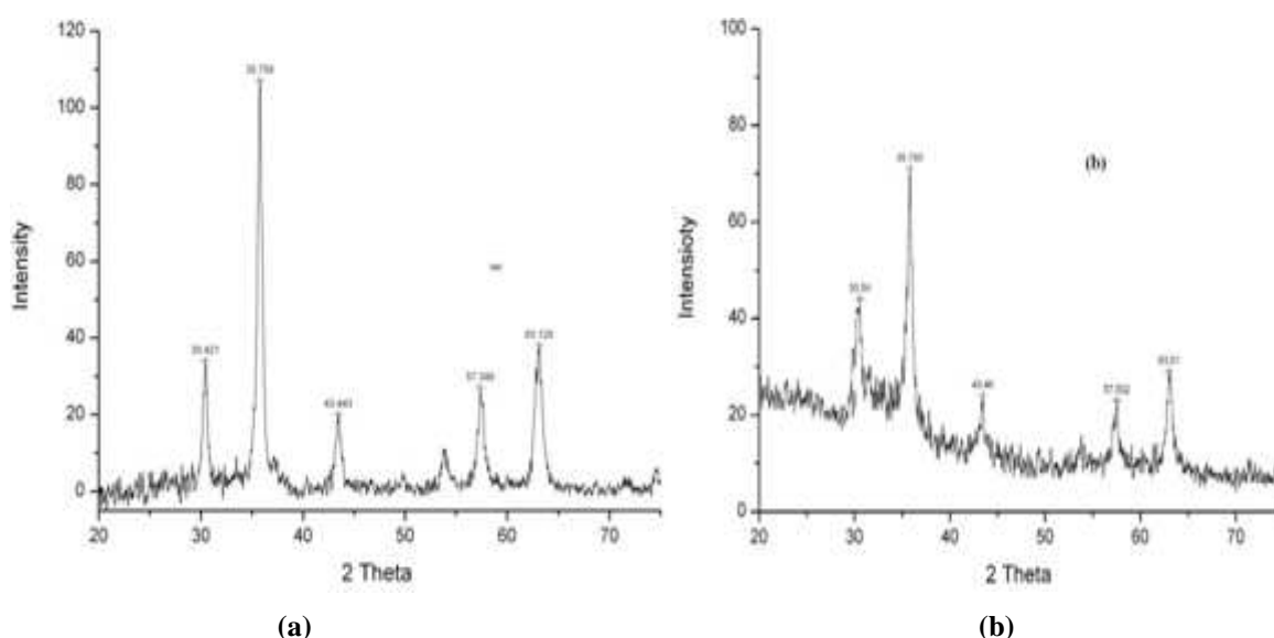
Figure 1: XRD Patterns of Olive (a) and Flaxseed (b) Oils Mediated SPIONs
