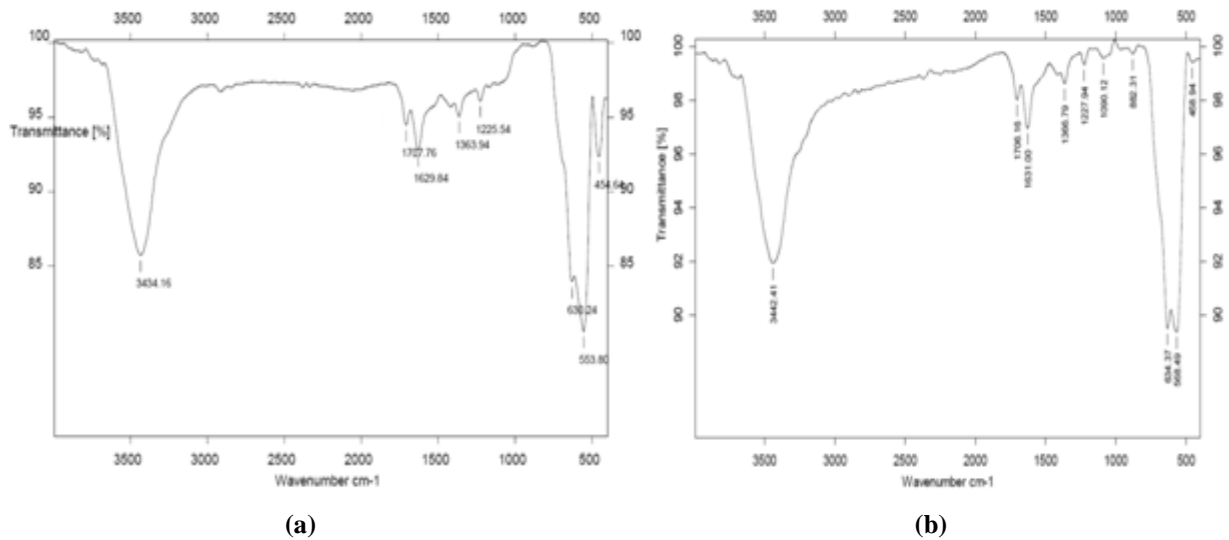
Figure 2: FTIR Analysis of MIONs a) Olive Oil Stabilized b) Flaxseed Oil Stabilized
