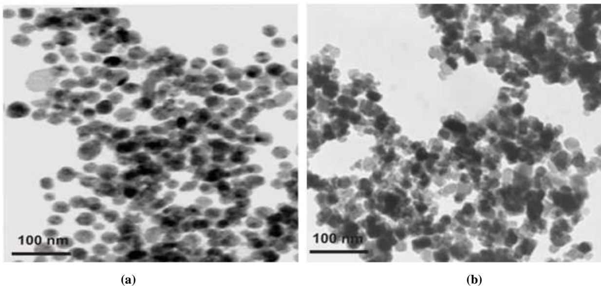
Figure 3: TEM Photographs of MIONs a) Olive Oil Stabilized b) Flaxseed Oil Stabilized
